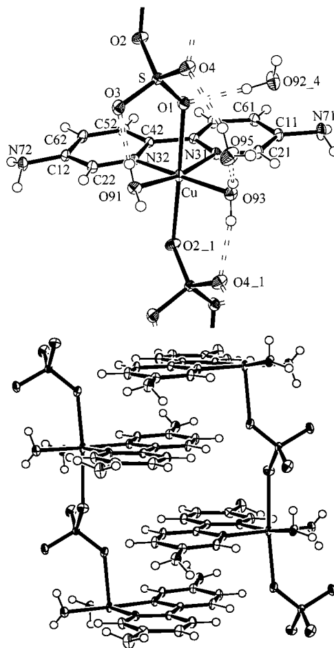
Figure 4. (a, top) Section of the one-dimensional coordination polymer [\text{Cu}(\mu\text{-SO}_4)(\mathbf{5})(\text{H}_2\text{O})_2] \times 3 \text{ H}_2\text{O} ( 19 ) indicating also part of the hydrogen bonding network with two water molecules of crystallization; selected distances [Å] and angles [°]: Cu–N31 2.010(2), Cu–N32 1.992(2), Cu–O91 2.006(2), Cu–O93 1.993(2), Cu–O1 2.468(2), Cu–O2#1 2.311(2); N32–Cu–O93 175.08(6), O91–Cu–N31 168.89(6), O1–Cu–O2#1 173.73(6), O93–Cu–O91 92.61(6), N32–Cu–N31 82.10(6), O1–Cu–N31 86.54(6), O1–Cu–O91 84.38(6), O91–Cu–O2#1 90.03(6), N31–Cu–O2 99.33(5), other angles between cis -positioned atoms range from 88.3 and 93.6° (symmetry equivalent position #1 = x - 1, y, z ; #4 = x - 0.5, -y + 0.5, z + 0.5 ); (b, bottom) \pi - \pi stacking of neighboring strands, running along a
