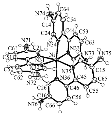
Figure 3. Exemplified view of the molecular structure of the tris(chelate)metal cations in [\text{Fe}(\mathbf{5})_3]\text{SO}_4 \times 9 \text{ H}_2\text{O} ( 16 ), [\text{Ni}(\mathbf{5})_3]\text{Cl}_2 \times 2.5 \text{ H}_2\text{O} ( 17 ), [\text{Ni}(\mathbf{5})_3](\text{SCN})_2 ( 18 , shown here), and in [\text{Zn}(\mathbf{5})_3](\text{NO}_3)_2 ( 22 ); selected distances and angles are given in Table 3
