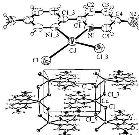
Figure 7. (a, top) Building block for the one-dimensional coordination polymer [\text{Cd}(\mu\text{-Cl})_2(\mathbf{5})] \times 2 \text{H}_2\text{O} ( 25 ) and (b, bottom) partial packing diagram which shows the formation of one-dimensional strands; the water molecules of crystallization have been omitted for clarity; selected distances [Å] and angles [°]: Cd-N1 2.332(8), Cd-Cl#3 2.561(8), Cd-Cl#5,7 2.78(1); N1-Cd-N1#3 70.2(4), N1-Cd-Cl 159.6(11), N1-Cd-Cl#7 96.5(2), Cl-Cd-Cl#3 103.2(3), N1#3-Cd-Cl 94.5(3), N1#3-Cd-Cl#7 85.8(2), Cl-Cd-Cl#7 95.7(3), Cl#3-Cd-Cl#7 82.5(3), Cl#7-Cd-Cl#5 177.17(4) (symmetry transformations: #3 = -x, y, -z + 0.5 ; #5 = -x, -y, -z ; #7 = x, -y, z + 0.5 )
